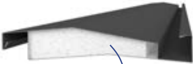
Louver Structure Sandwich construction with Peripor core
